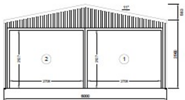
4 FRONT ELEVATION 2 SCALE: 1:50 FRAME #1
